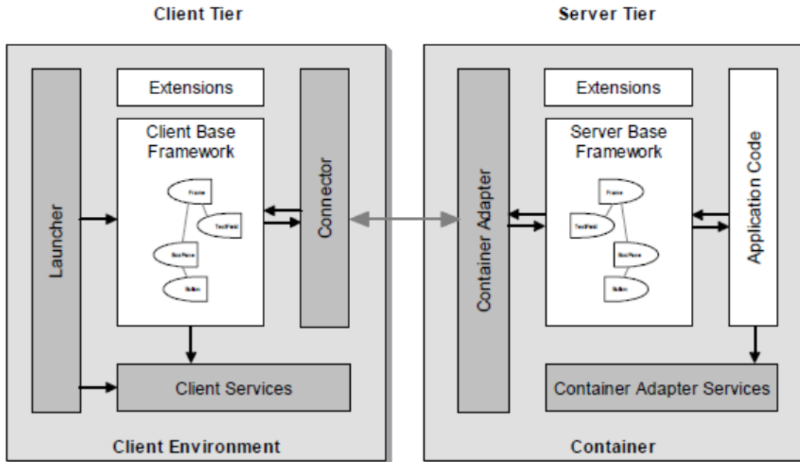
Figure 1: Technical architecture overview
